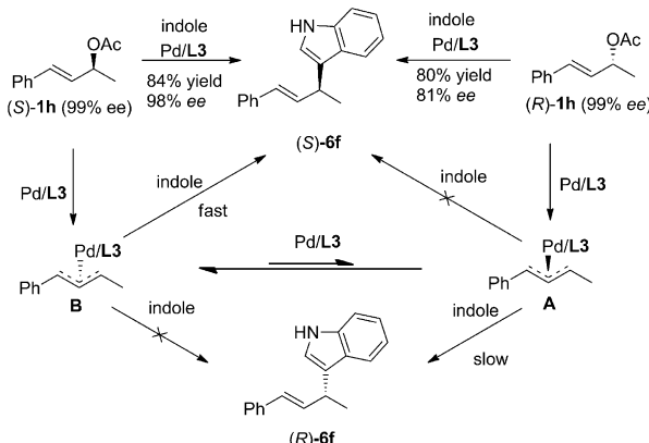
Scheme 2. The transformation of optically pure 1h catalyzed by [\text{PdCl}(\text{C}_3\text{H}_5)_2]_2/\text{L3} .
