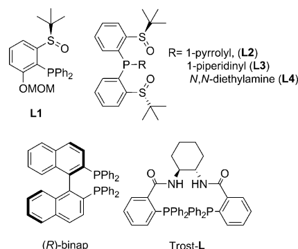
Figure 1. Chiral ligands used in this work. MOM = methoxymethyl.
